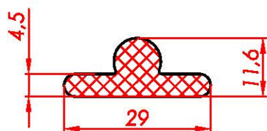
676 60ShA
