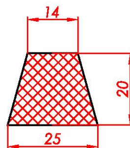
630 60ShA
