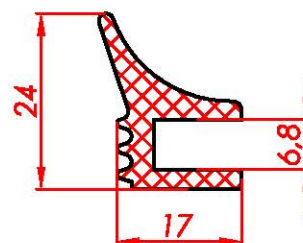
660 70ShA
