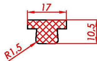
565 60ShA
