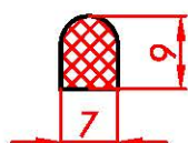
956 65/80ShA
