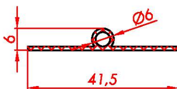
086 60ShA
