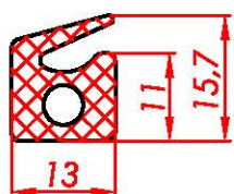
864 60ShA
