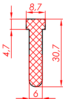
811 60ShA
