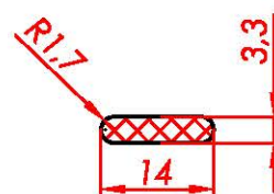
609 60ShA
