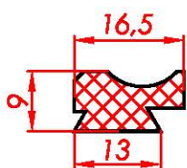
952 75ShA
