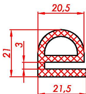
008 60ShA
