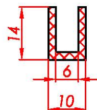
224 60ShA
